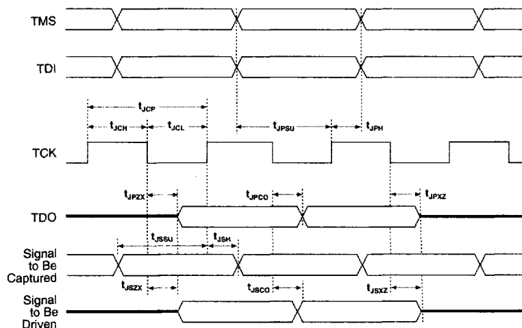
Figure 17. JTAG Waveforms
